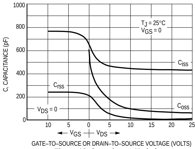
Figure 16. Capacitance Variation
