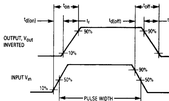
Figure 14. Switching Waveforms
