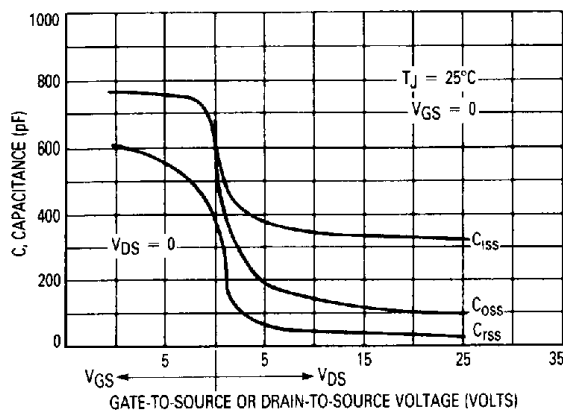
Figure 11. Capacitance Variation
