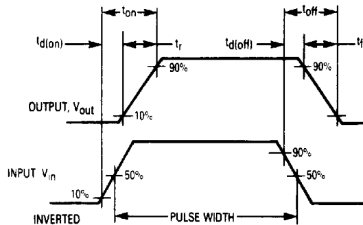
Figure 13. Switching Waveforms
