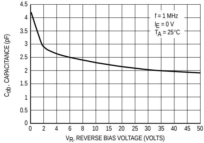
Figure 39. Output Capacitance
