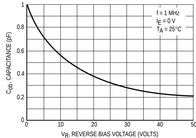
Figure 29. Output Capacitance
