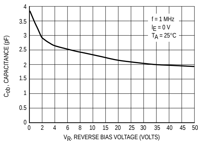
Figure 34. Output Capacitance
