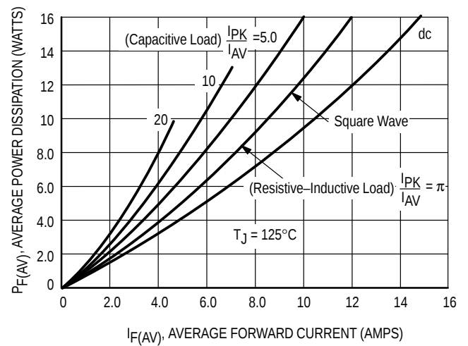
Figure 15. Power Dissipation
