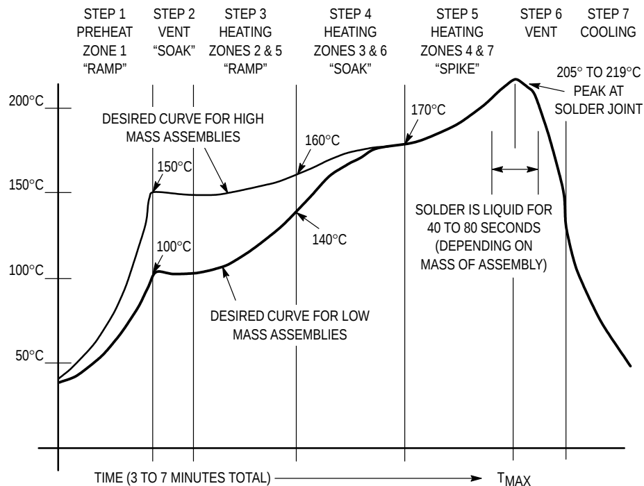
Figure 7. Typical Solder Heating Profile for D 2 PAK
