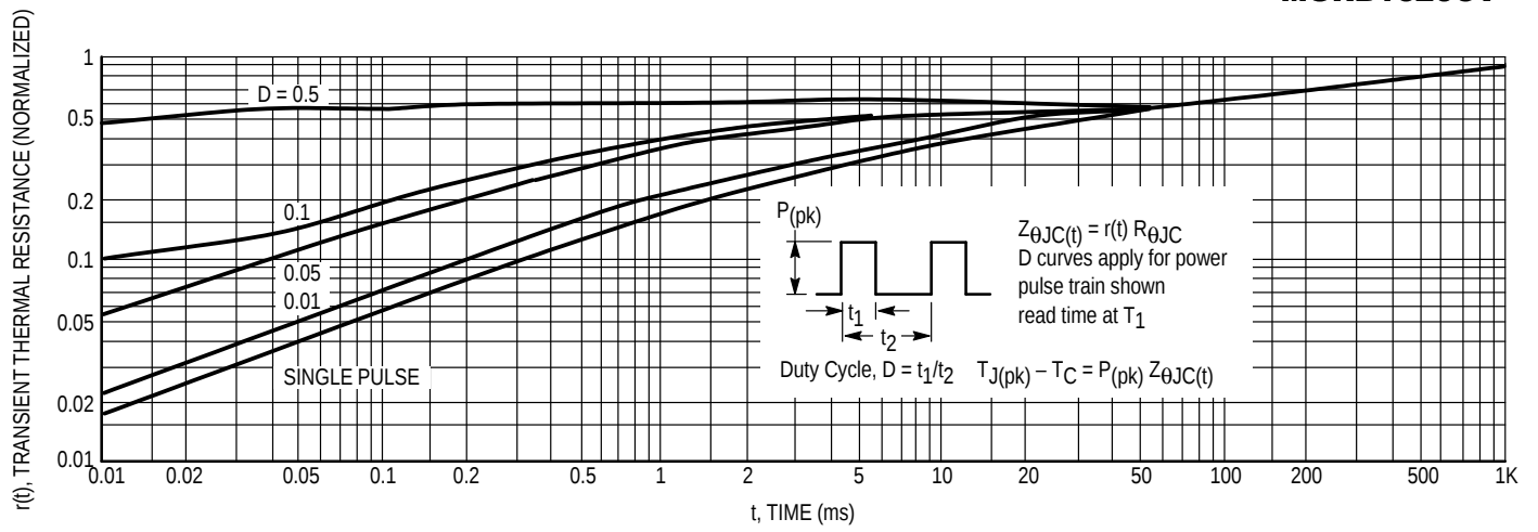
Figure 5. Thermal Response
