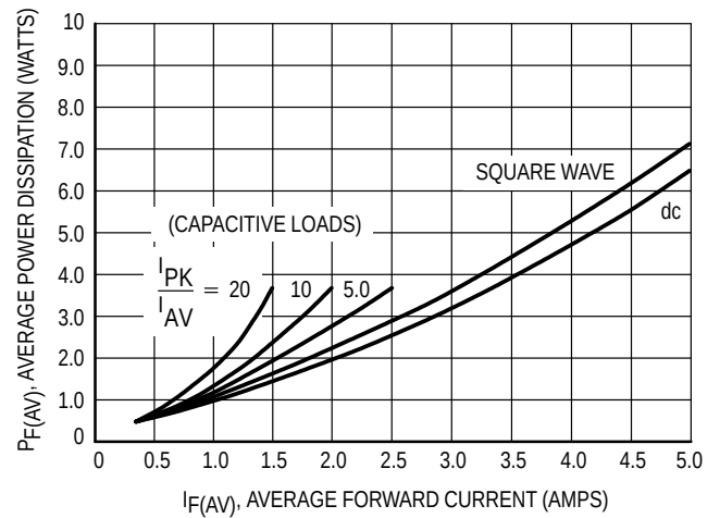
Figure 8. Power Dissipation
