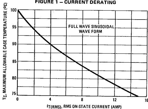
FIGURE 1 – CURRENT DERATING
