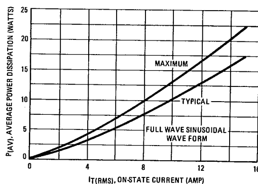
FIGURE 2 – POWER DISSIPATION
