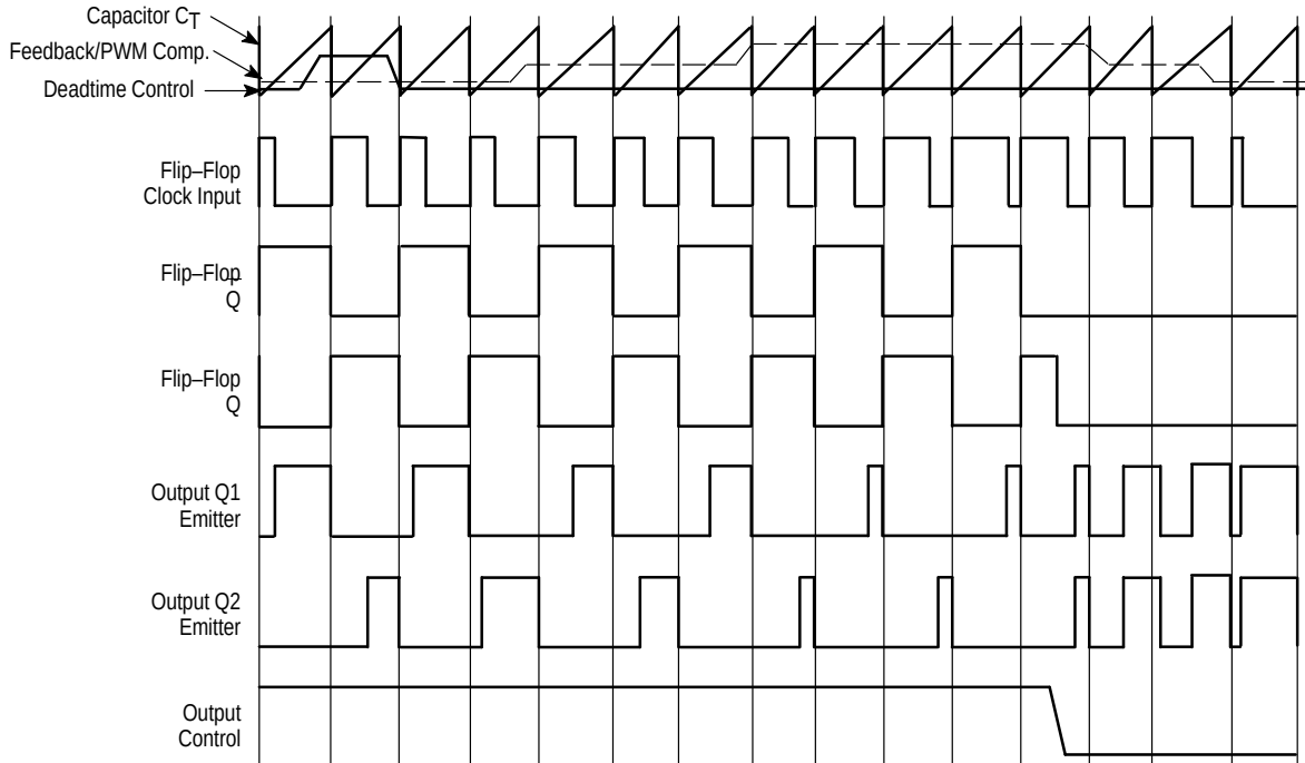
Figure 2. Timing Diagram
