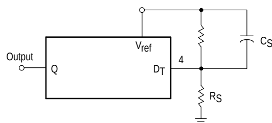
Figure 17. Soft-Start Circuit
