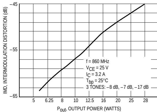
Figure 1. IMD versus Output Power
