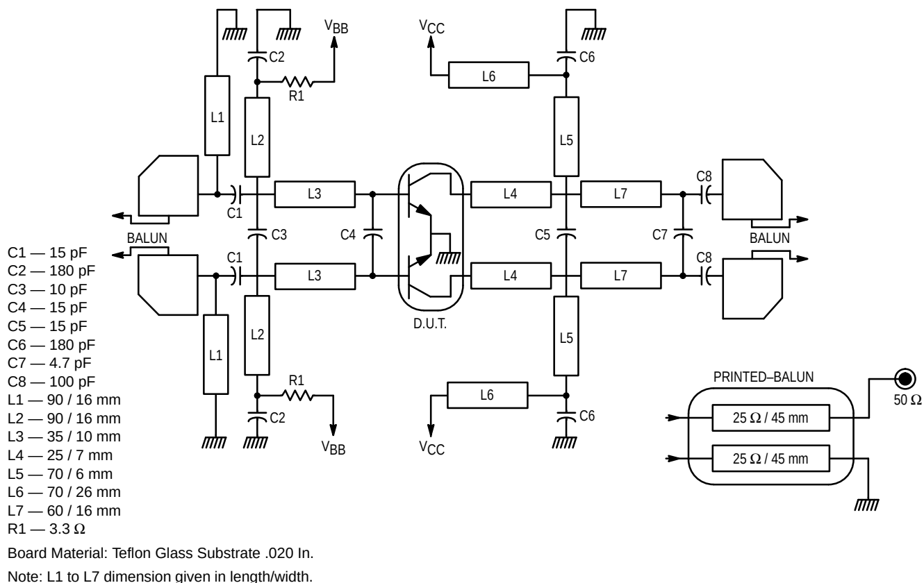
Figure 3. 470–860 MHz Broadband Test Circuit
