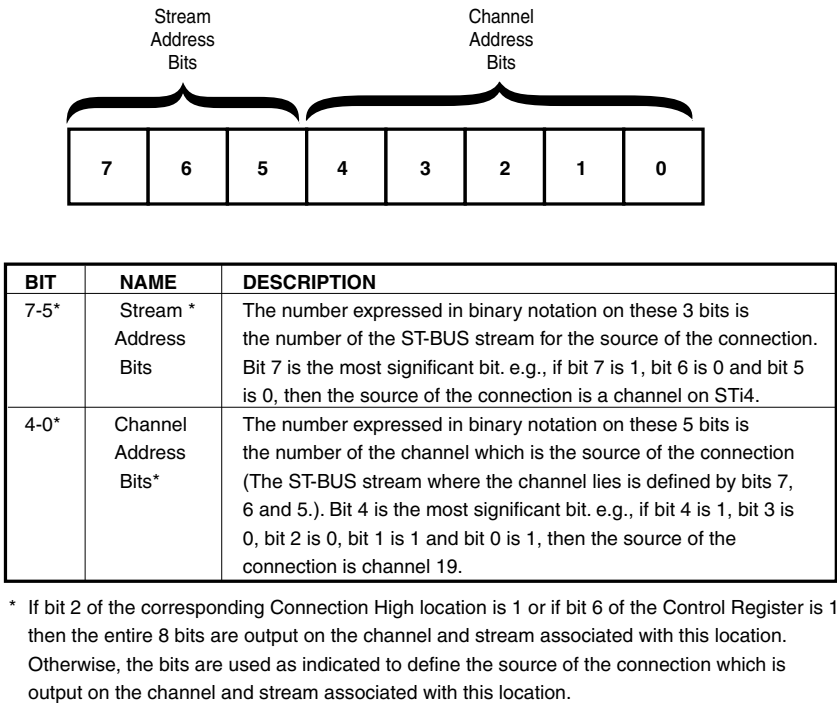
Figure 6 - Connection Memory Low Bits
