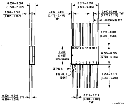
16-Lead Ceramic Flatpak (F) NS Package Number W16A
