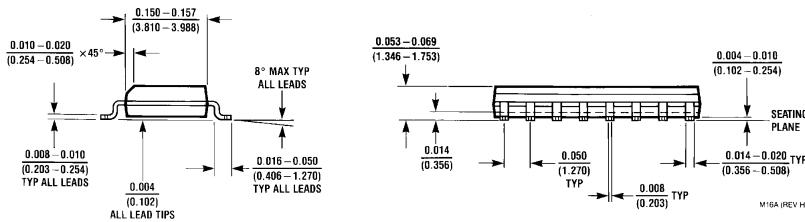
16 Lead Small Outline Ingrated Circuit (S) NS Package Number M16A
