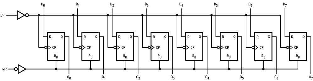
Logic Diagram
