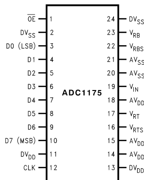
ADC1175 Pin Configuration
