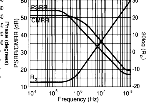
PSRR, CMRR, and Closed Loop R_o
