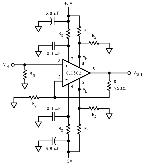
FIGURE 3. Location of Damping Resistors ( R_Q )
