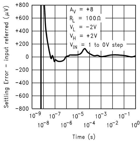
Long-Term Settling, Clamped (4x overdrive)
