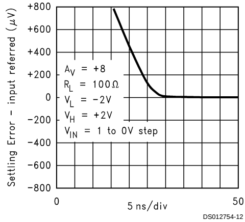
Settling, Clamped (4x overdrive)
