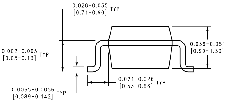
5-Pin SOT23 NS Package Number MA05A
