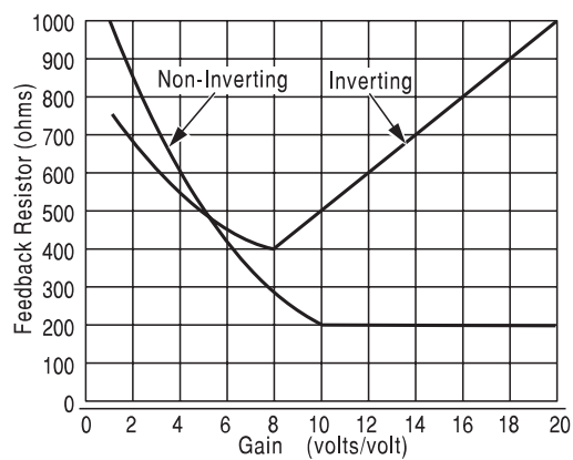
Recommended R_f vs. Gain (CLC431)
