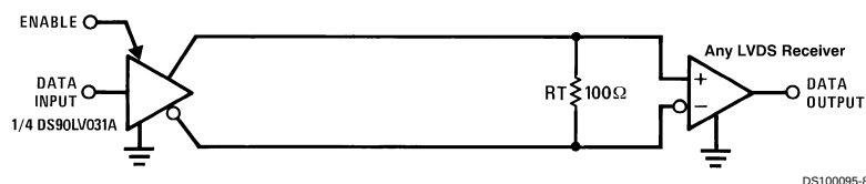
FIGURE 6. Point-to-Point Application
