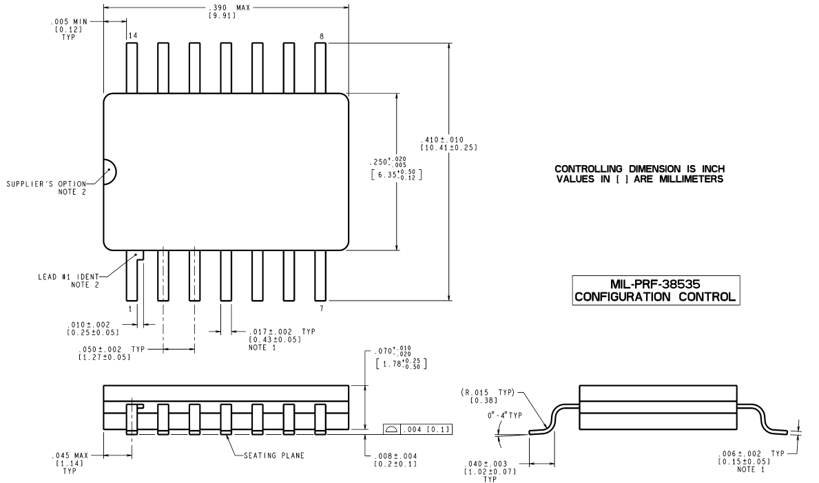
14-Pin Ceramic Package (WG) NS Package Number WG14A
