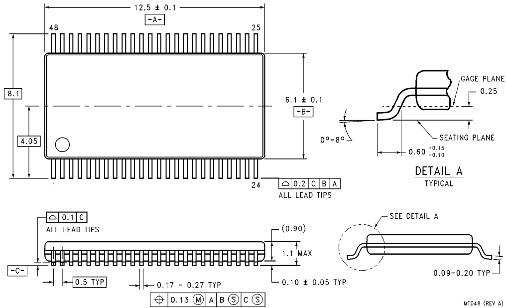
48-Lead Thin Shrink Small Outline Package, JEDEC, 6.1 mm Body Width Order Number 74LCX16373MTD or 74LCX16373MTDX NS Package Number MTD48
