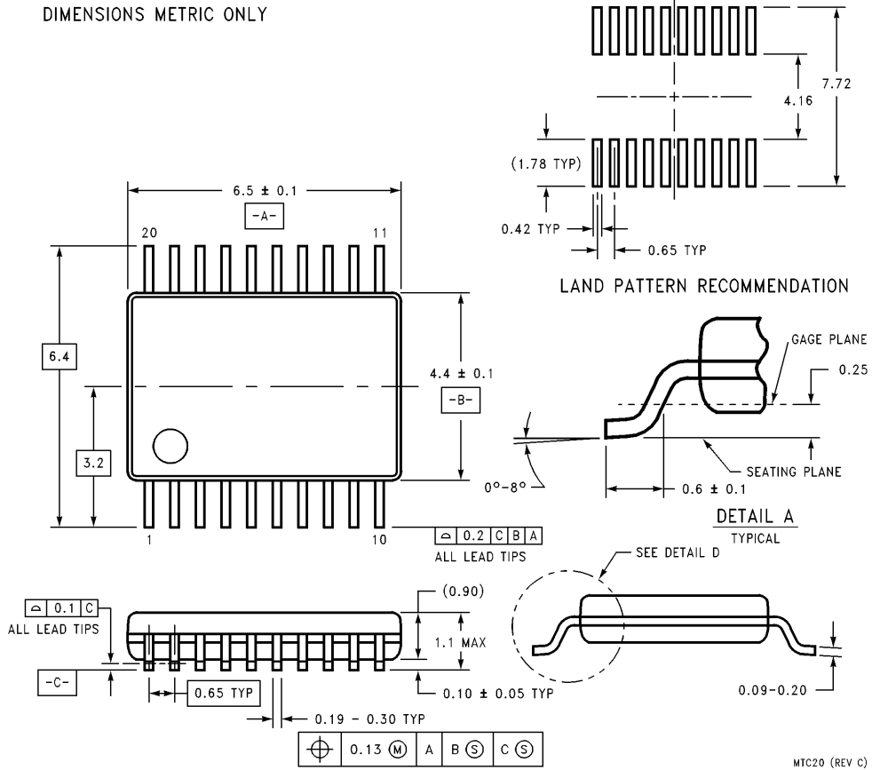
20-Lead Molded Thin Shrink Small Outline Package, JEDEC Order Number 74LVT244MTC or 74LVT244MTCX NS Package Number MTC20
