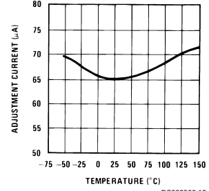
Adjustment Current
