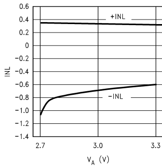
INL vs V_A
