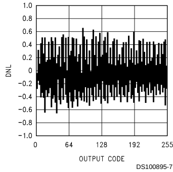
DNL @ 42 MSPS
