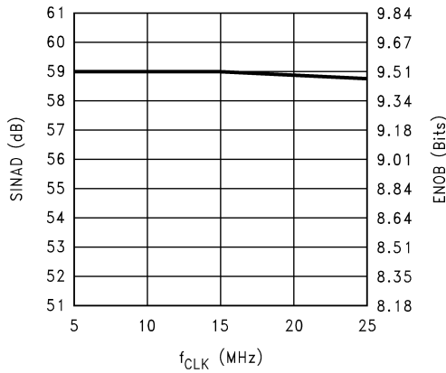
SINAD & ENOB vs. @ f_{CLK} ( f_{IN} = 9.5 MHz)
