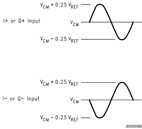
FIGURE 2. The ADC10D020 is designed for use with differential signals of 1.0 V_{P-P} with a common mode voltage of 1.5V. The signal swing should not cause any pin to experience a swing more than 300 mV beyond the supply rails.
