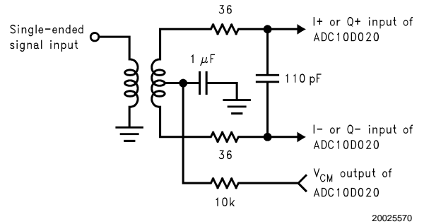
FIGURE 3. Use of an input transformer for single-ended to differential conversion can simplify circuit design for single-ended signals.
