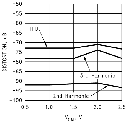
Distortion vs. V_{CM} @ f_{IN} = 4.7\text{ MHz}
