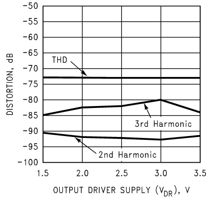
Distortion vs. V_{DR} @ f_{IN} = 4.7\text{ MHz}
