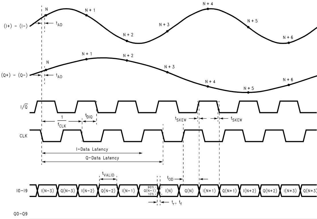
ADC10D020 Timing Diagram for Multiplexed Mode
