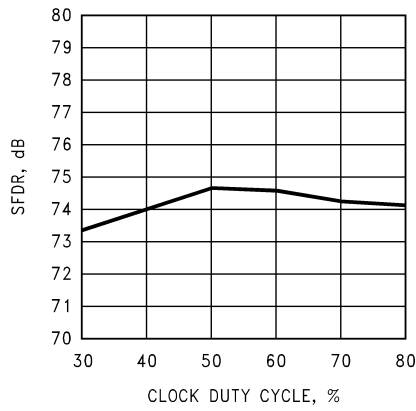
SFDR vs. Clock Duty Cycle @ f_{IN} = 4.7 MHz
