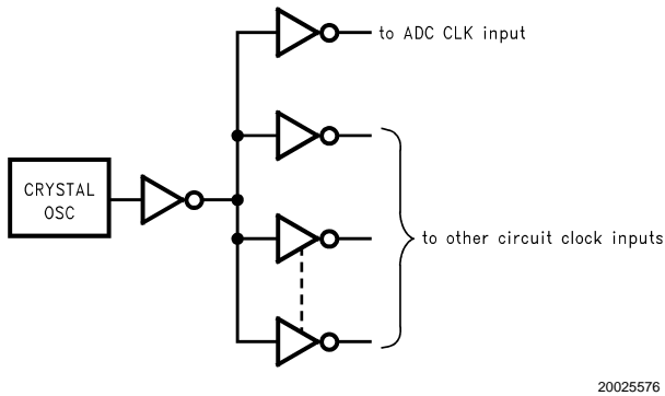
FIGURE 9. Isolating the ADC Clock from Digital Circuitry
