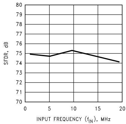
SFDR vs. f_{IN}
