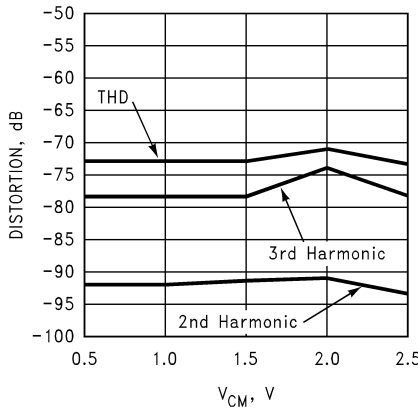
Distortion vs. V_{CM} @ f_{IN} = 4.7 MHz
