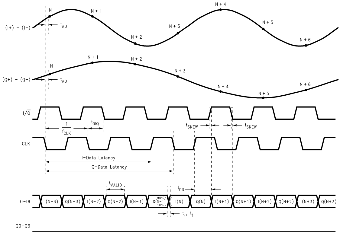
ADC10D040 Timing Diagram for Multiplexed Mode
