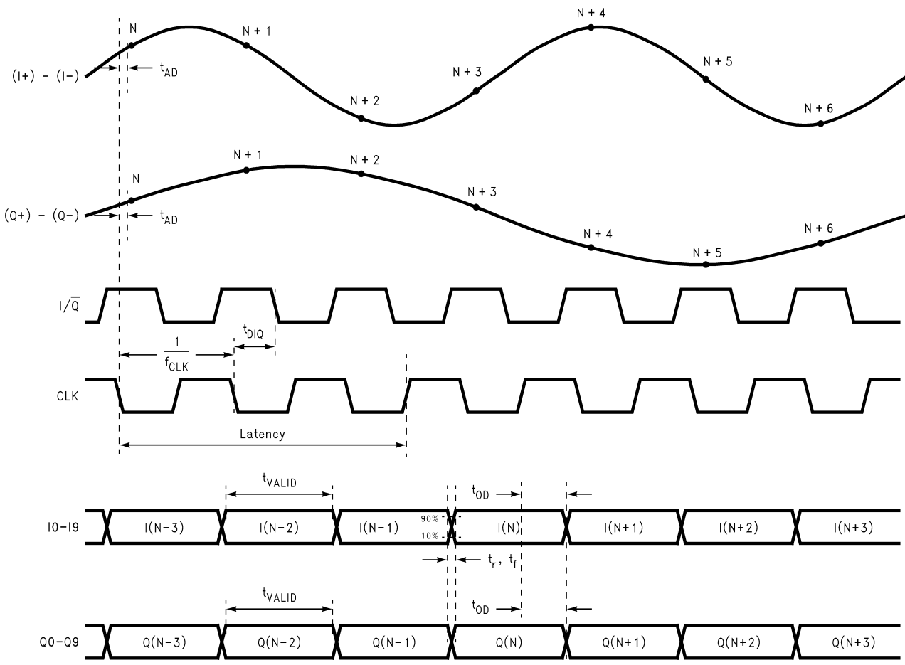
ADC10D040 Timing Diagram for Parallel Mode
