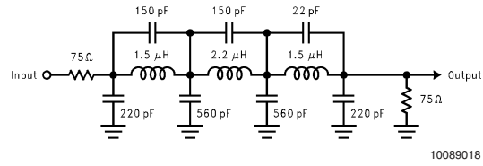
FIGURE 8. 5.5 MHz Low Pass Filter to Eliminate Harmonics at the Signal Input.
