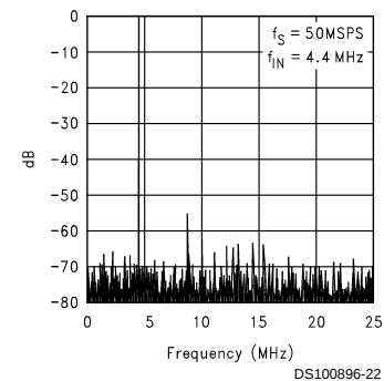
Spectral Response
