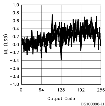
INL Plot
