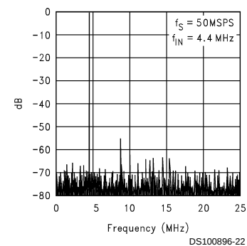
Spectral Response
