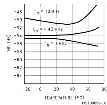
THD vs Temp & f_{IN}
