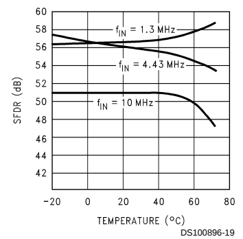
SFDR vs Temp & f_{IN}
