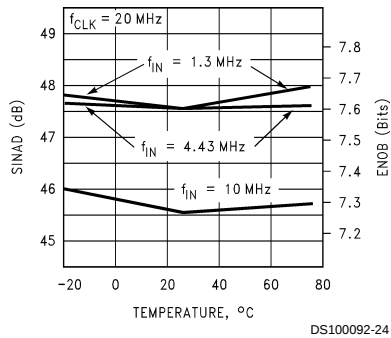
SINAD/ENOB vs Temp
