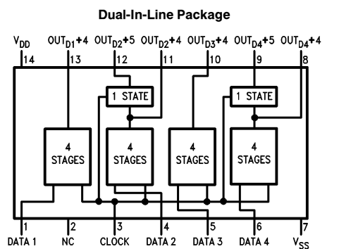
Top View Order Number CD4006B
