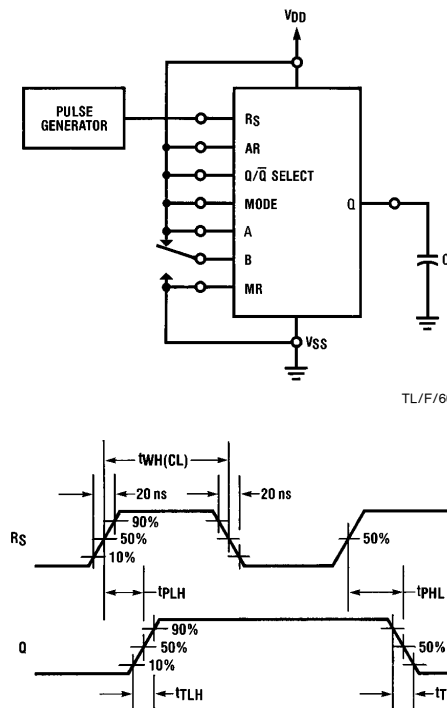
Switching Time Test Circuit and Waveforms
