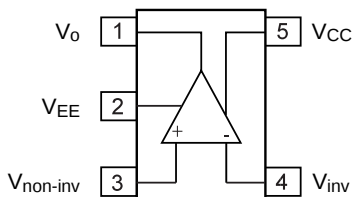
PINOUT SOT23-5
