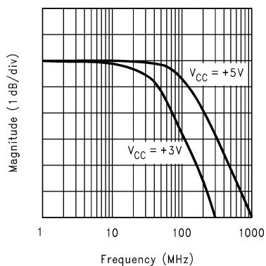
Small Signal Bandwidth
