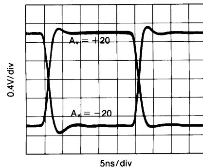
Pulse Response
