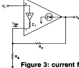
Figure 3: current feedback topology
