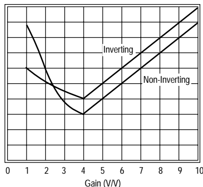
Figure 4: Recommended R_f vs. Gain
