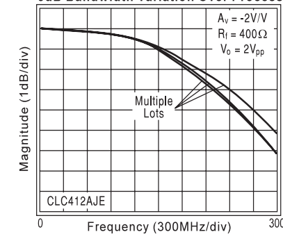
-3dB Bandwidth Variation Over Process
