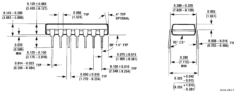
14-Pin MDIP NS Product Number N14A
