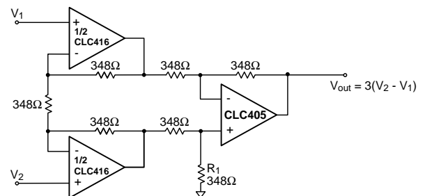
Figure 4: Instrumentation Amplifier
