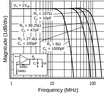
Recommended R_s vs. Capacitive Load
