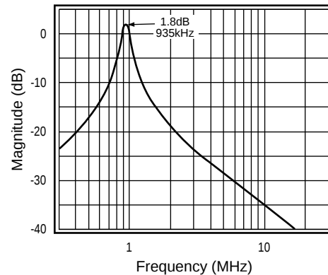
Figure 7: Bandpass Response
