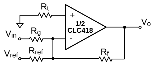
Figure 4: Level Shifting Circuit
