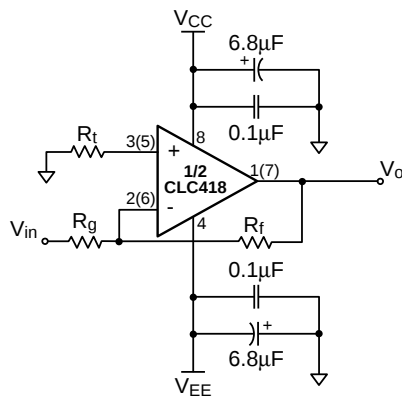
Figure 2: Inverting Gain
