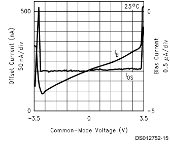
I B and I OS vs. Common-Mode Voltage
