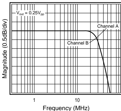
Figure 6: Channel Matching
