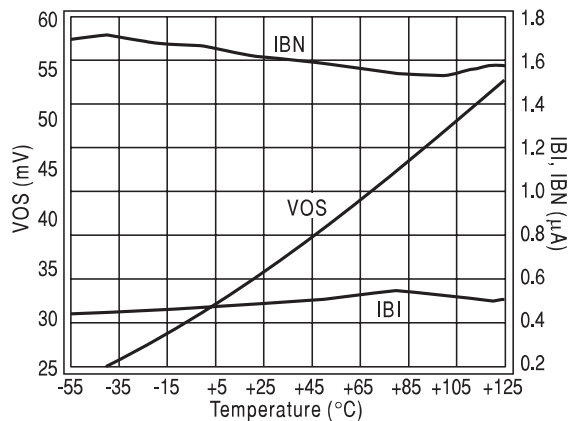
Typical DC Errors vs. Temperature
