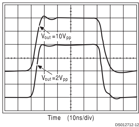
Pulse Response
