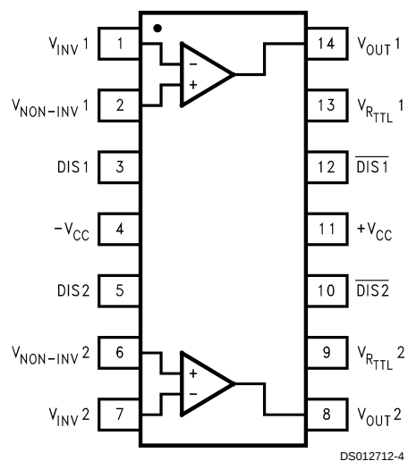
Pinout CLC431 DIP & SOIC
