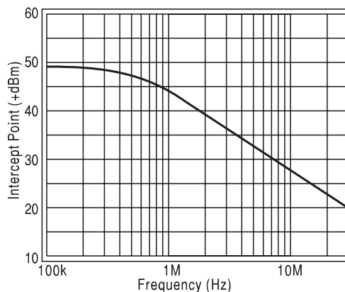
2-Tone, 3rd-Order Intermod. Intercept
