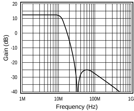
Figure 12: Ideal Elliptic Filter Frequency Response
