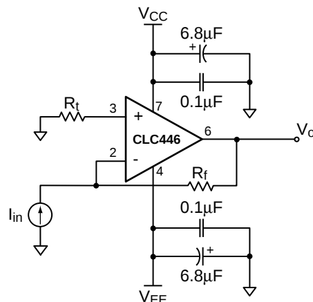
Figure 3: Transimpedance Gain
