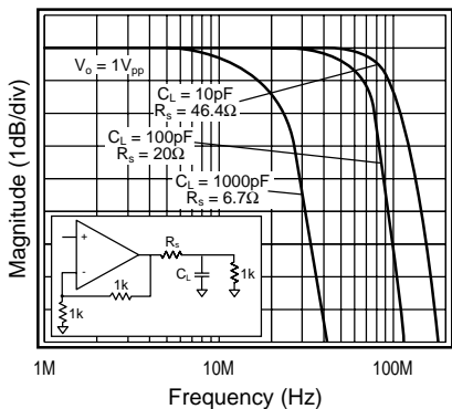
Figure 7: Frequency Response vs. C_L
